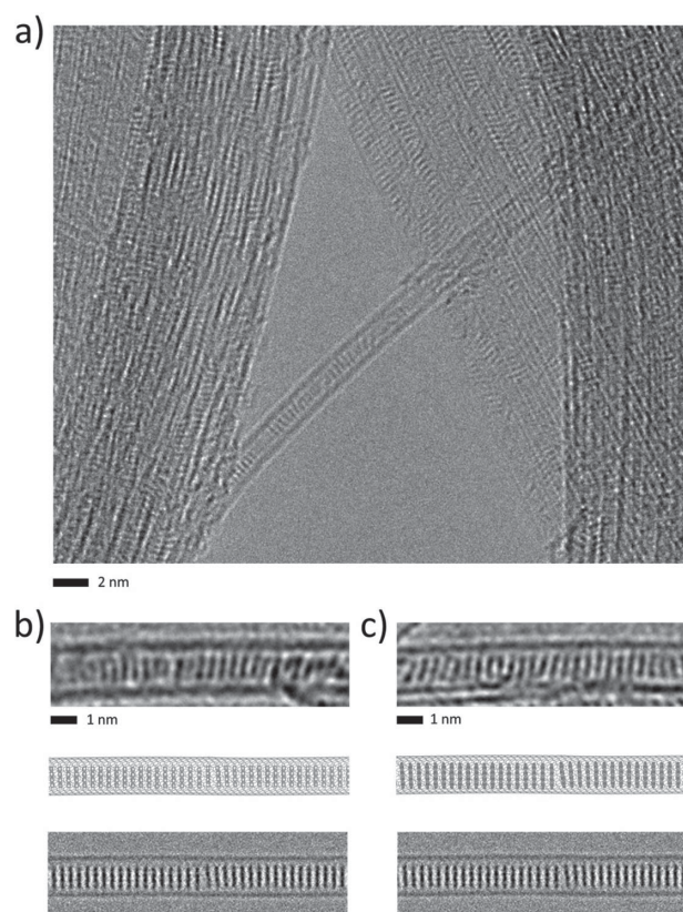
Figure 5. a) AC-HRTEM image of coronene- \text{d}_{12} @SWNT demonstrating excellent filling rates. b,c) Comparison of AC-HRTEM images, corresponding structural models and image simulations for coronene@SWNT (b) and coronene- \text{d}_{12} @SWNT (c) showing that the structures are essentially identical.
