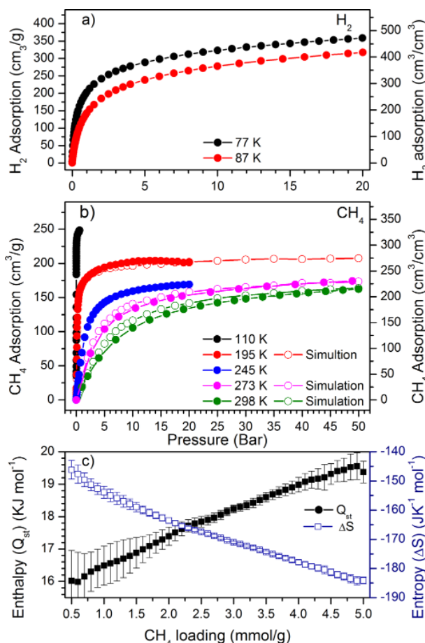
Figure 1. (a,b) Adsorption isotherms of \text{H}_2 and \text{CH}_4 in MFM-300(In), respectively. (c) Variation of the isosteric heat ( Q_{\text{st}} ) and entropy ( \Delta S ) of adsorption of \text{CH}_4 in MFM-300(In).
